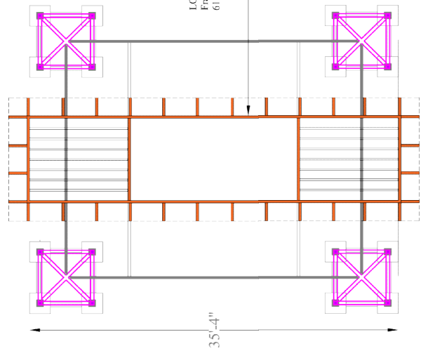
ENTRANCE ARCHWAY LOW LEVEL FRAMING
