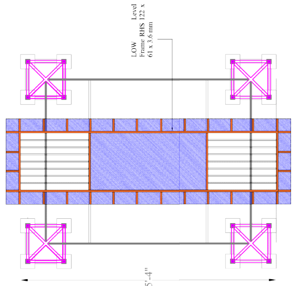
ENTRANCE ARCHWAY ACP CLADDING DETAIL
