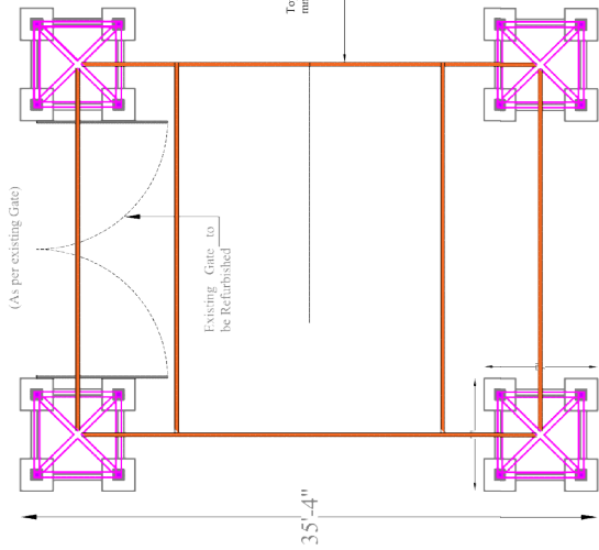
ENTRANCE ARCHWAY TOP LEVEL FRAMING
